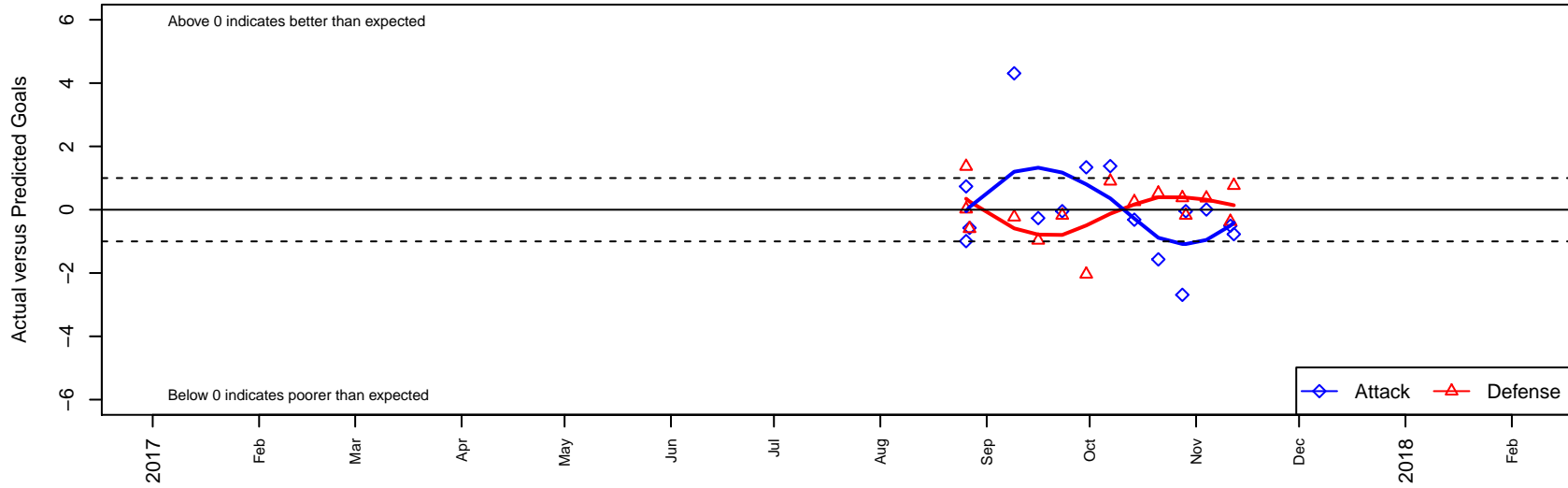
Crossfire OR SSC White G05 Dots are actual minus expected GF (blue circles) and GA (red triangles). Blue line is smoothed change in attack strength. Red is smoothed change in defense strength.
